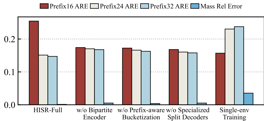
(b) Prefix-level & Mass Metrics
