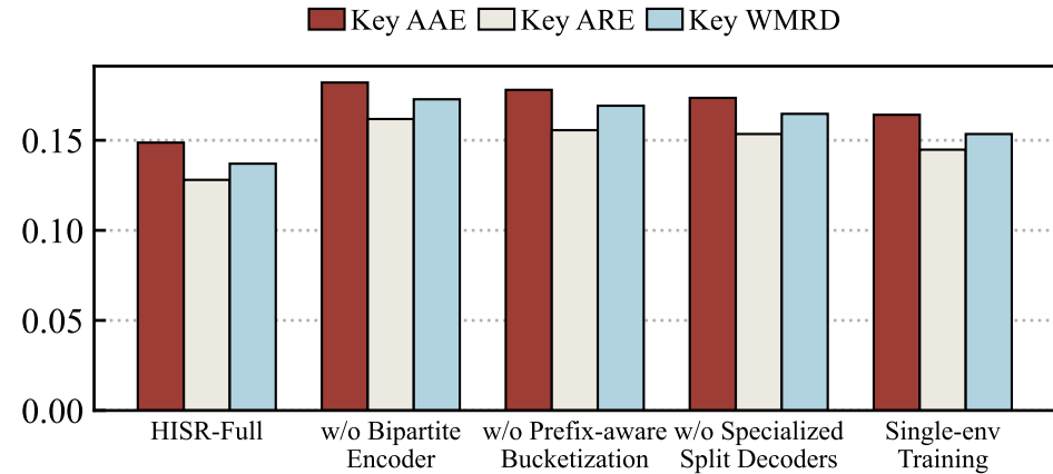
(a) Key-level Metrics
