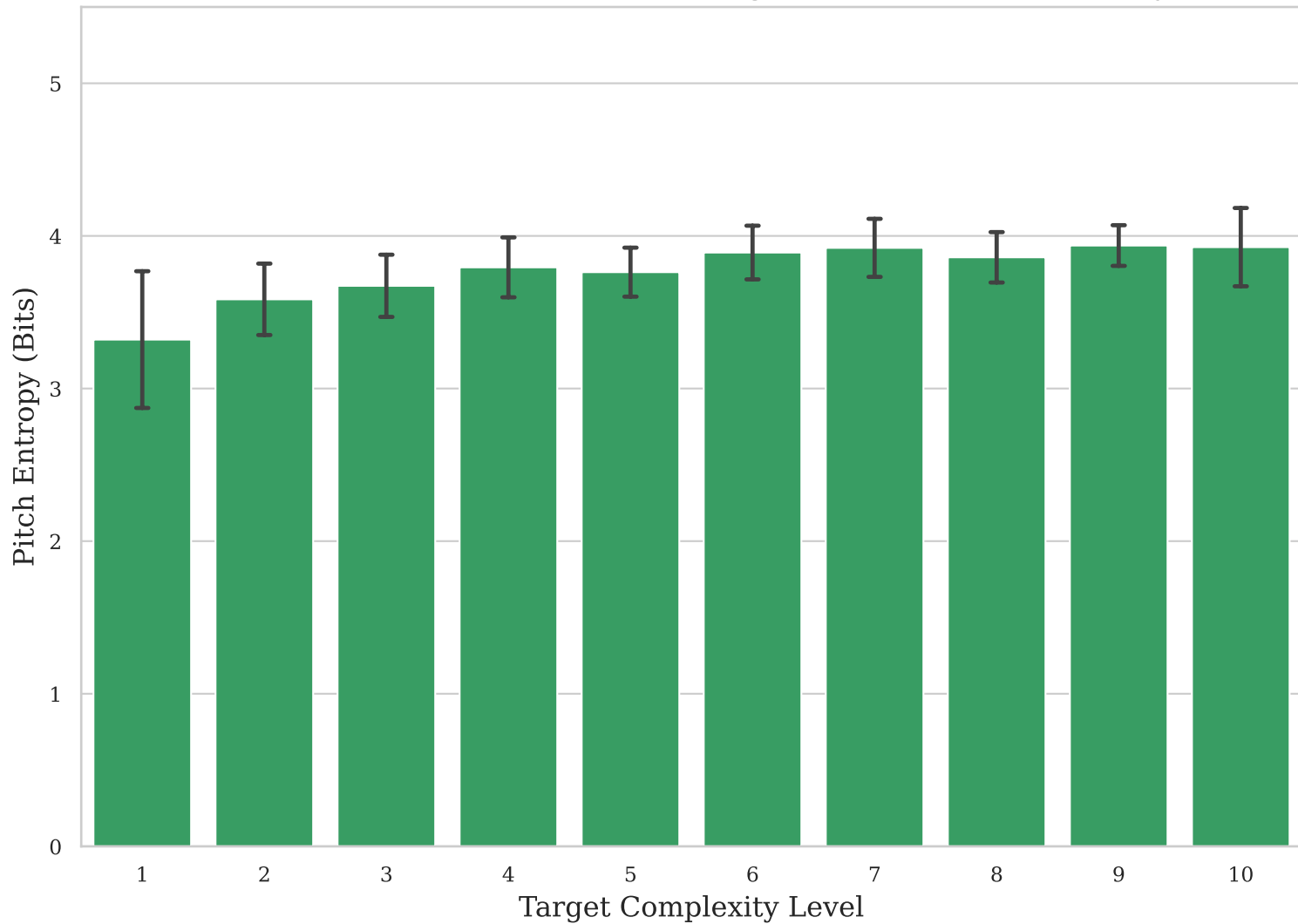
Verification of Feature Decoupling (Pitch Shannon Entropy)
