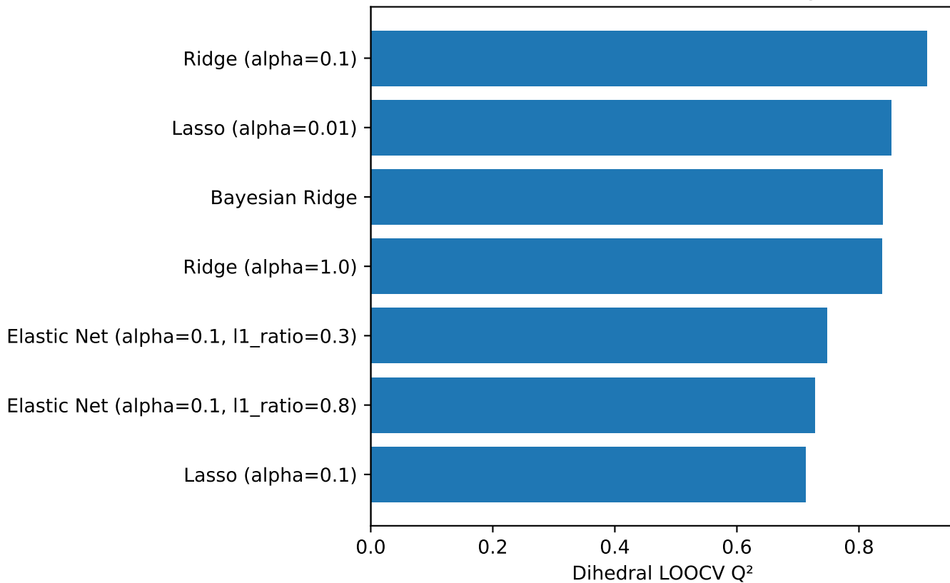
Reaction C method ranking
