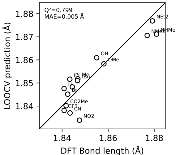
Bond length: \sigma p+
