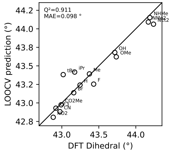
Dihedral: \sigma p+
