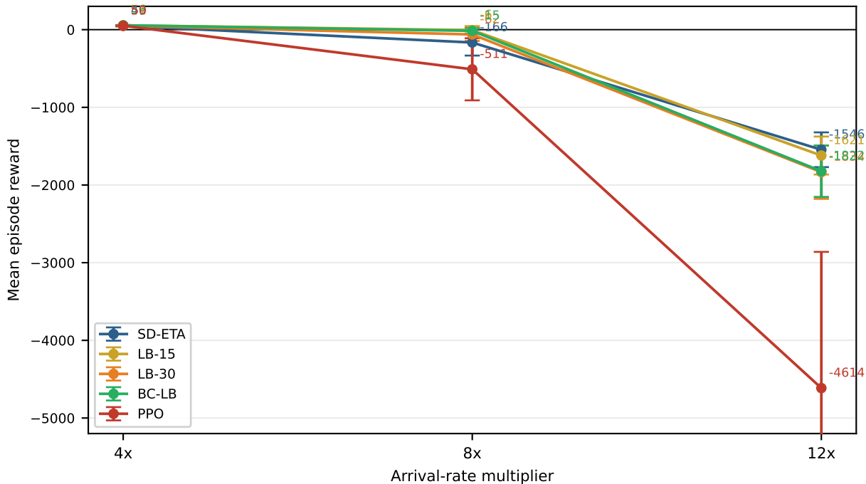
Density regime under the main weight distribution
