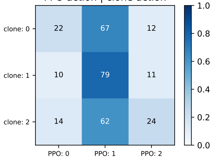
PPO action | clone action
