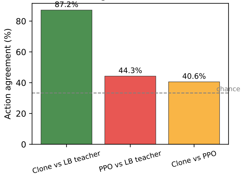
Decision agreement (seed 9999)
