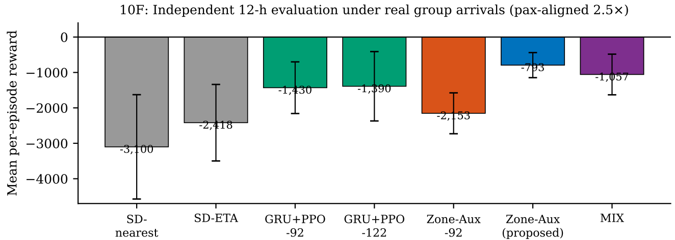
FIGURE 2. Independent 12-hour evaluation at 2.5× peak arrival rates (mean per-episode reward ± SE). Rule baselines (gray) collapse; the proposed Zone-Aux agent (blue) achieves -793 \pm 354 (3-seed pooled, n = 36 ) at the shortest waiting time, under the real group-arrival protocol.
