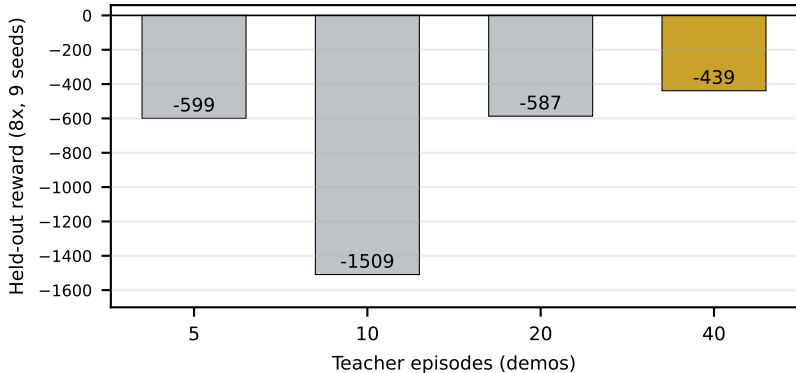
BC data efficiency (SD-ETA teacher)
