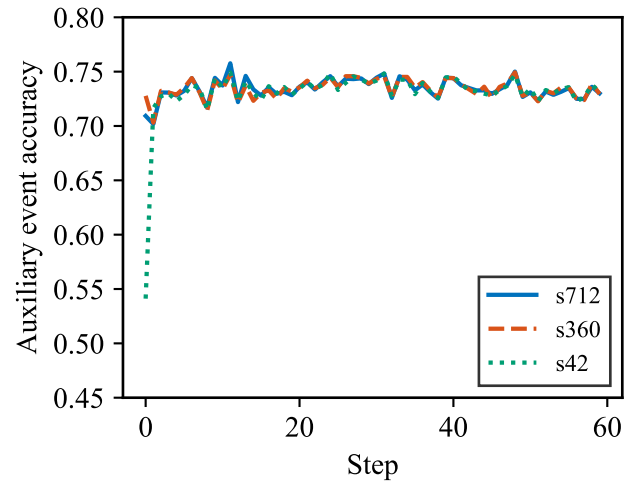
FIGURE 3. Auxiliary next-event zone-prediction accuracy during training (3 seeds). Accuracy reaches 0.70–0.73 against a 0.48 majority-class baseline (all-day event distribution).
