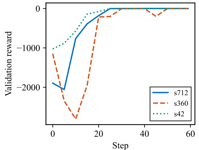
FIGURE 4. Training-internal validation reward (3 seeds; illustrative only, not used for cross-run comparison).
