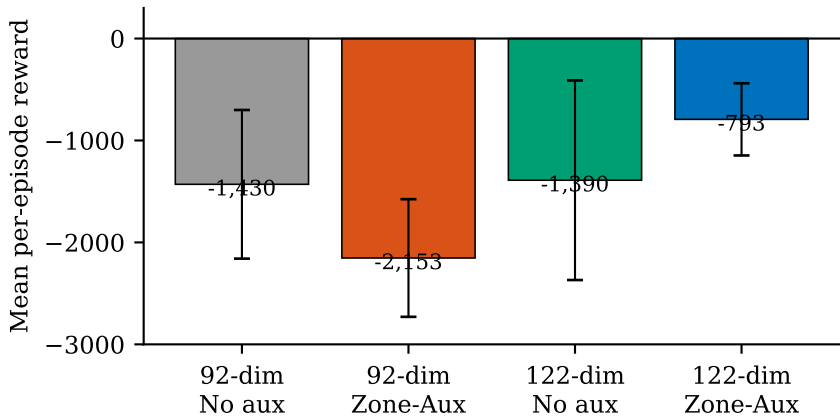
Feature \times auxiliary cross-ablation (group protocol)
