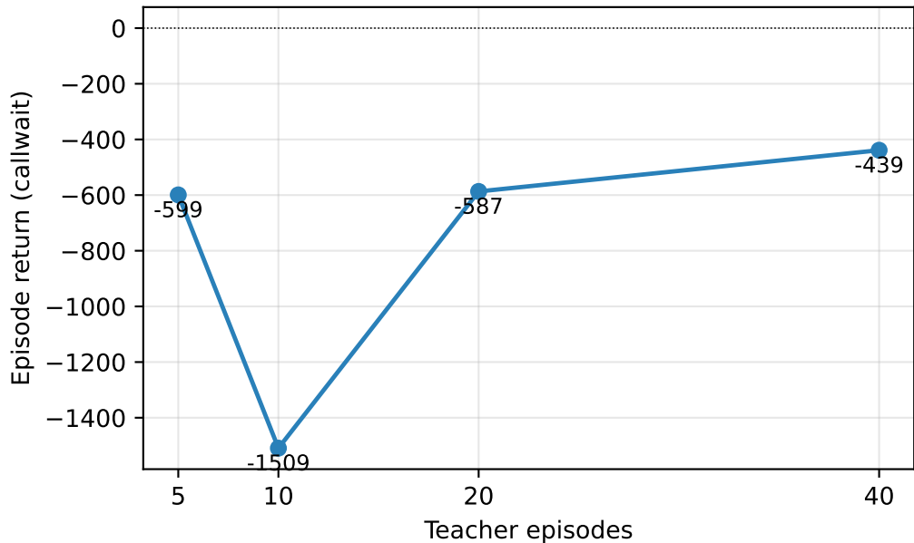
BC data efficiency (SD-ETA teacher, epoch 20, nine seeds)
