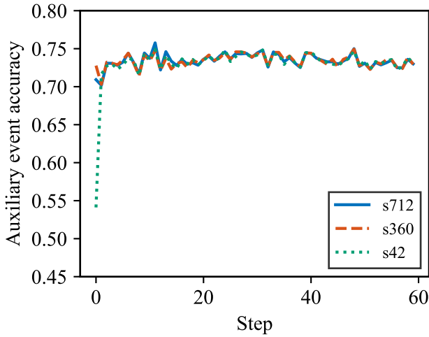
FIGURE 5. Auxiliary next-event zone-prediction accuracy during training (3 seeds). Accuracy reaches 0.70–0.73 against a 0.48 majority-class baseline (all-day event distribution).
