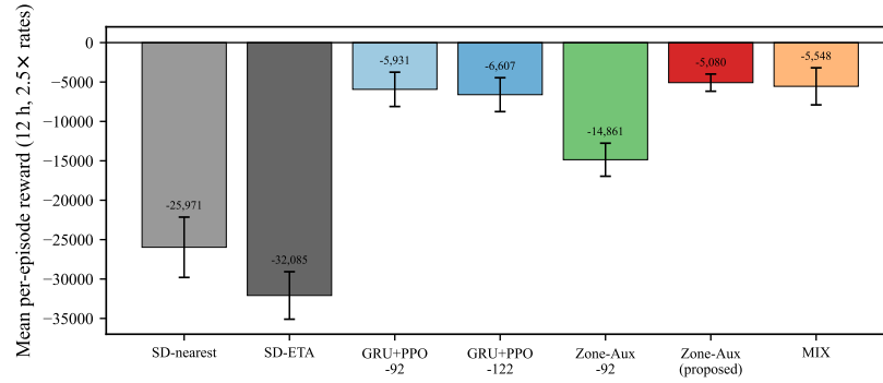
FIGURE 2. Independent 12-hour evaluation at 2.5\times peak arrival rates (mean per-episode reward \pm SE). Rule baselines (gray) collapse; the proposed Zone-Aux agent (red) achieves -5,080 \pm 1,090 (3-seed pooled, n = 36 ) with the shortest waiting time.
