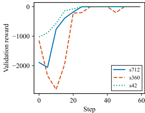
FIGURE 6. Training-internal validation reward (three seeds; illustrative only).
