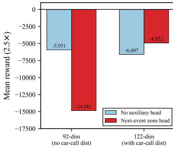
FIGURE 4. Feature \times auxiliary cross-ablation ( 2.5\times , seed 42): the next-event zone head helps only when the observation carries the car-call distribution (122-dim).
