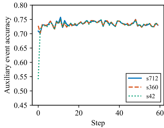
FIGURE 5. Auxiliary next-event zone-prediction accuracy during training (three seeds); accuracy reaches 0.70–0.73 against a 0.48 majority-class baseline.
