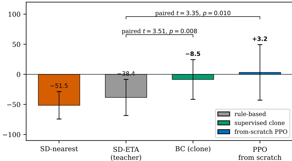
Mean 12-h episode reward
