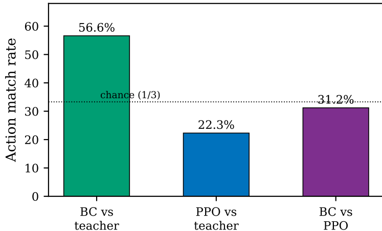
Decision agreement on shared teacher rollouts
