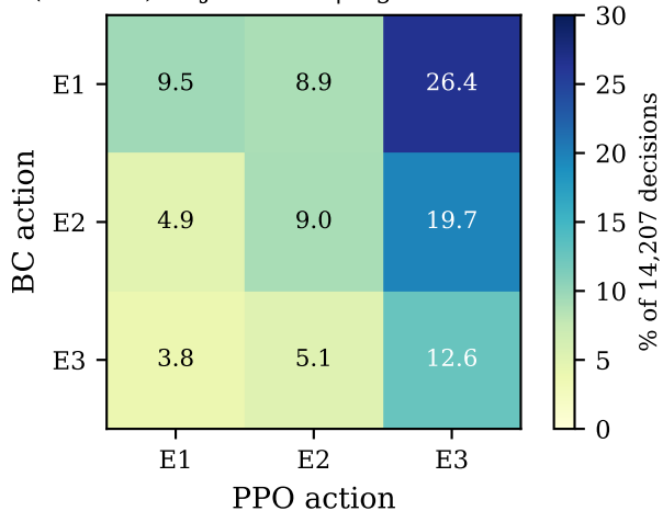
Joint decisions on teacher (SD-ETA) trajectories | agreement 31.2%
