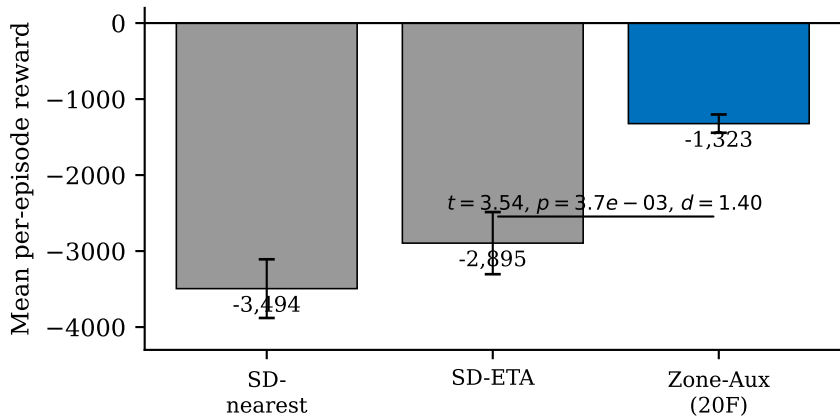
20F: 10F-trained agent under real group arrivals (2.5× pax-aligned)
