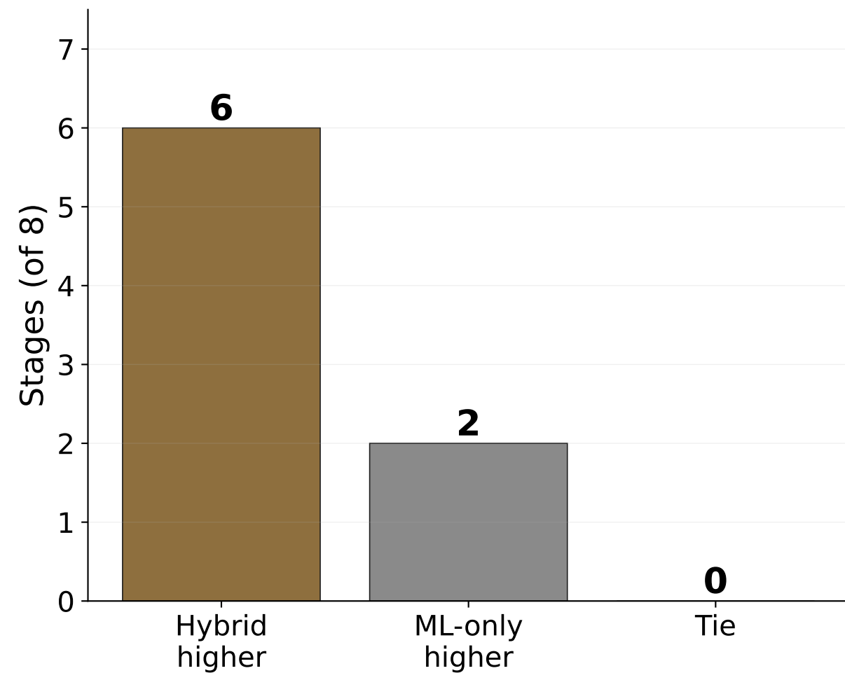
B. Hybrid higher in 6/8 (best-vs-best; mean \Delta R^2 = +0.03 )
