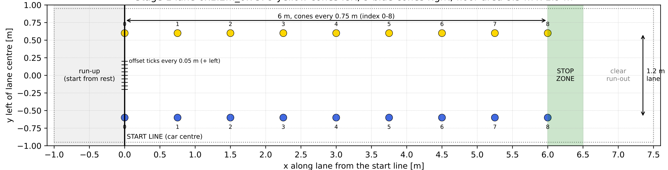
Stage 1 lane 6x1.2m_0.75: 9 yellow cones left, 9 blue cones right; floor area 8.5 m x 1.9 m
