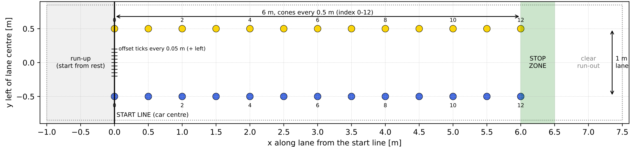
Stage 1 lane 6x1m_0.5: 13 yellow cones left, 13 blue cones right; floor area 8.5 m x 1.7 m
