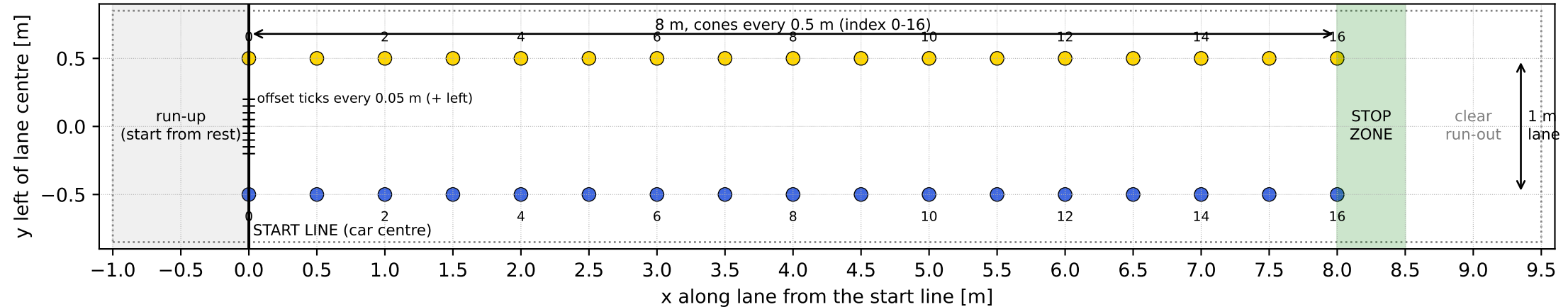
Stage 1 lane 8x1m_0.5: 17 yellow cones left, 17 blue cones right; floor area 10.5 m x 1.7 m
