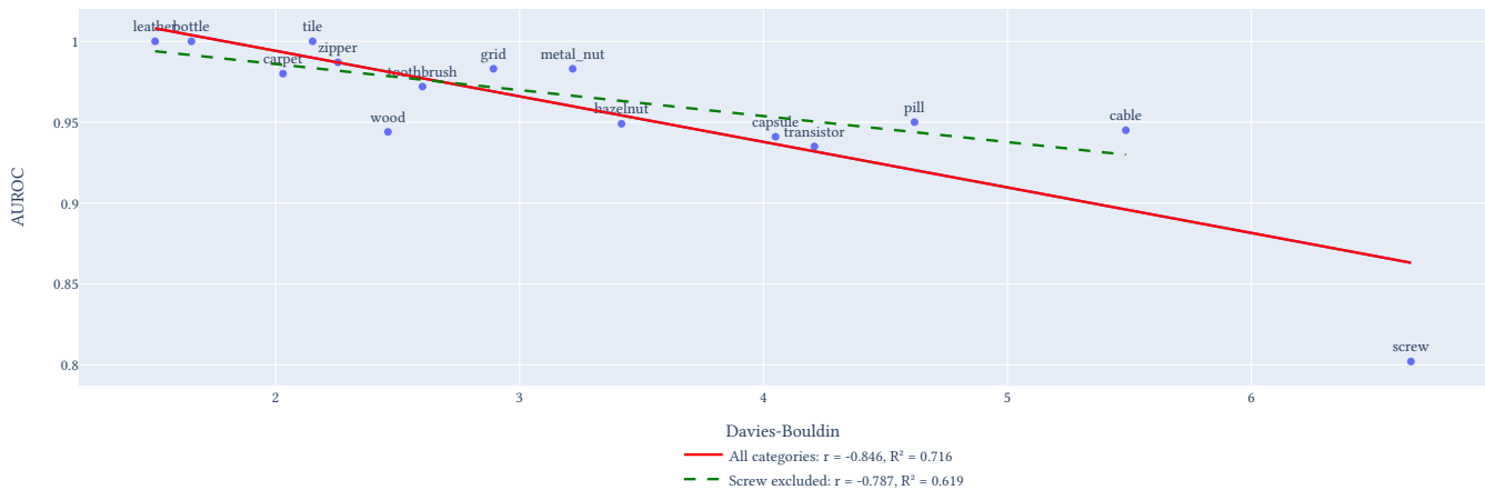
Figure 18: Davies-Bouldin Index vs AUROC
