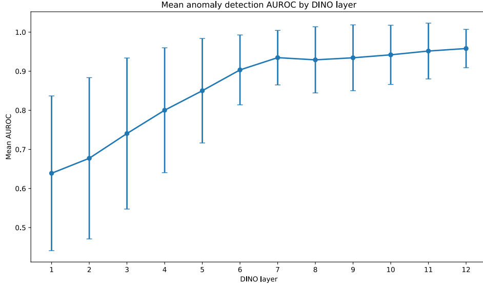
Figure 7: AUROC across DINO layers
