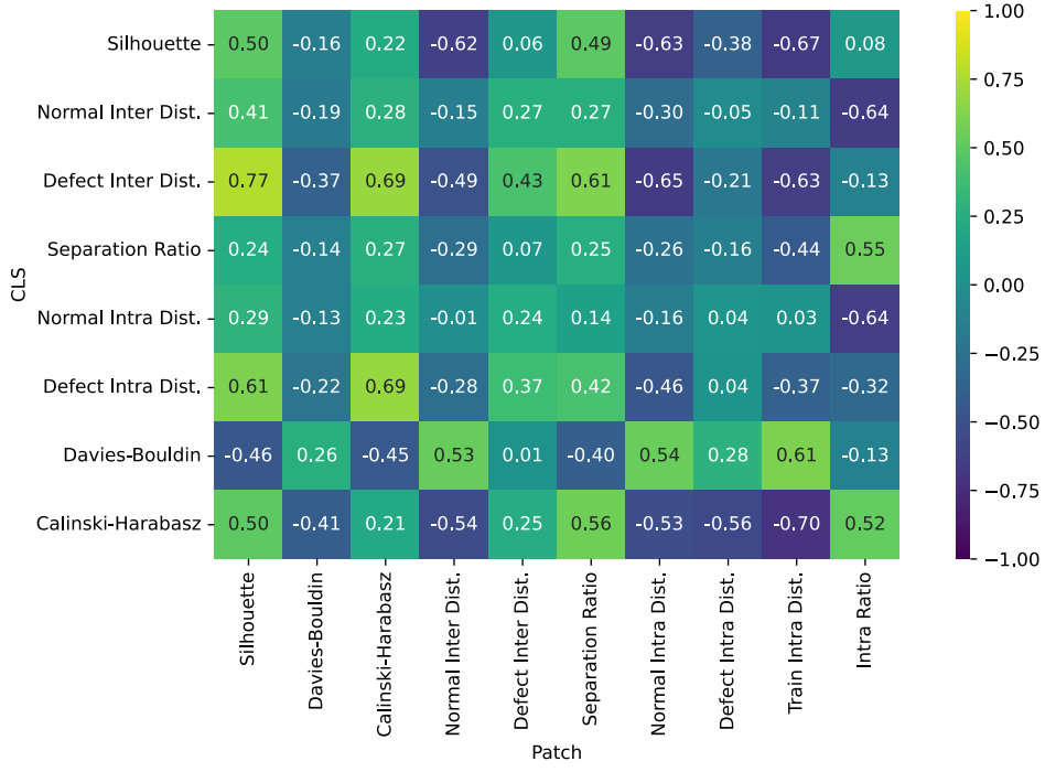
Figure 23: Correlation matrix between CLS and Patch metrics
