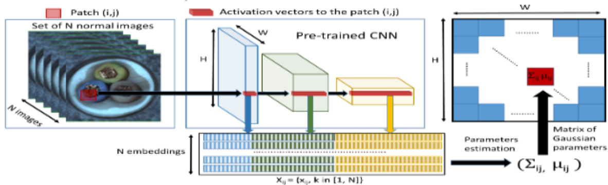
Figure 8: Architecture of PaDiM
