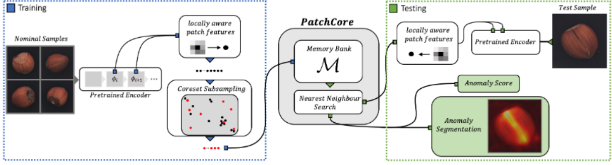
Figure 9: Architecture of Patchcore
