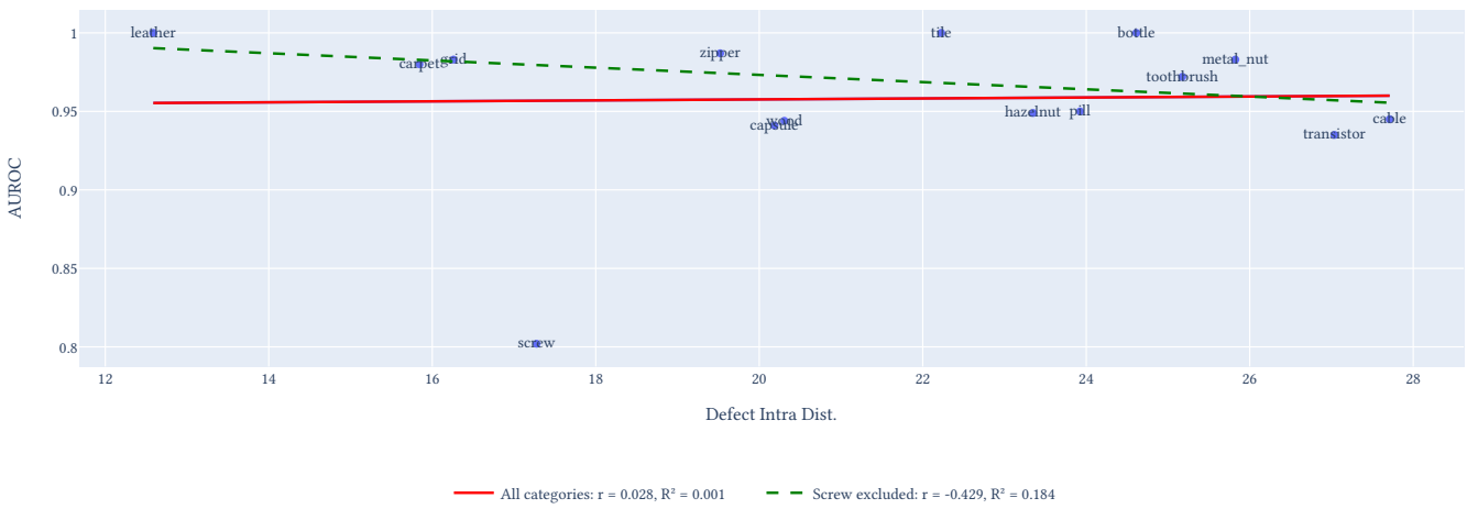
Figure 22: AUROC vs Defect Intra Distance
