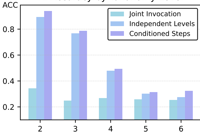
A: Accuracy by Taxonomy Level
