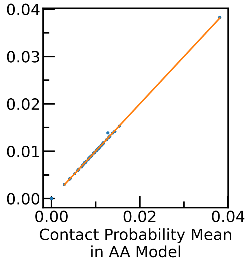
Contact Probability Mean in ME Model
