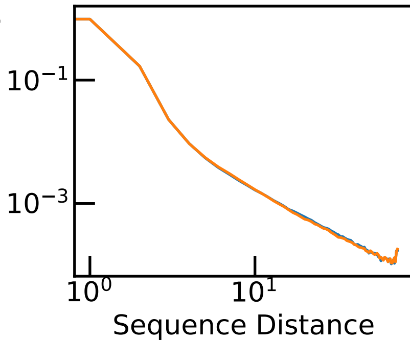
The 2-th Moment of Contance Probability
