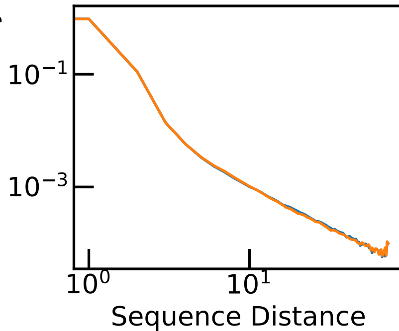
The 3-th Moment of Contance Probability
