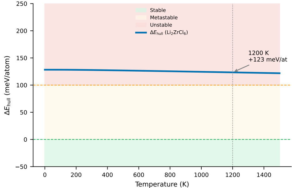
Hull distance vs temperature
