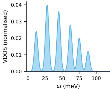
(a) Harmonic phonon DOS
