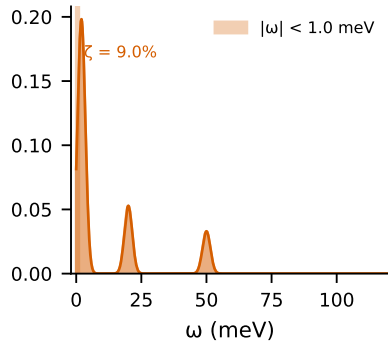
(c) Soft-mode signature
