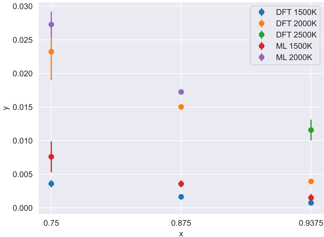
Mean and Std for DFT and ML at Different Temperatures
