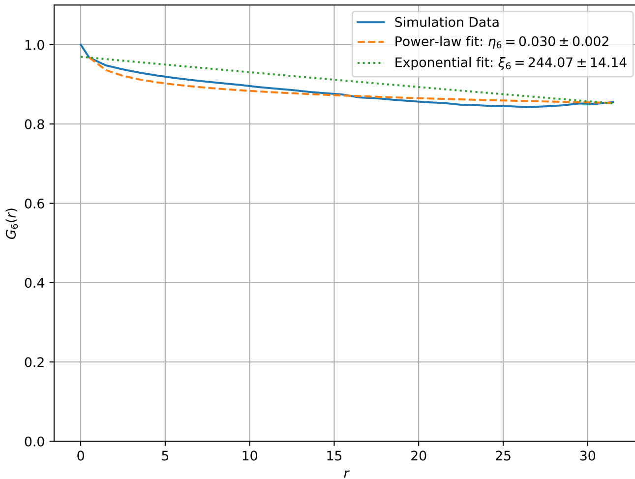
Correlation Function at T = 1.00e - 01 , L = 64
