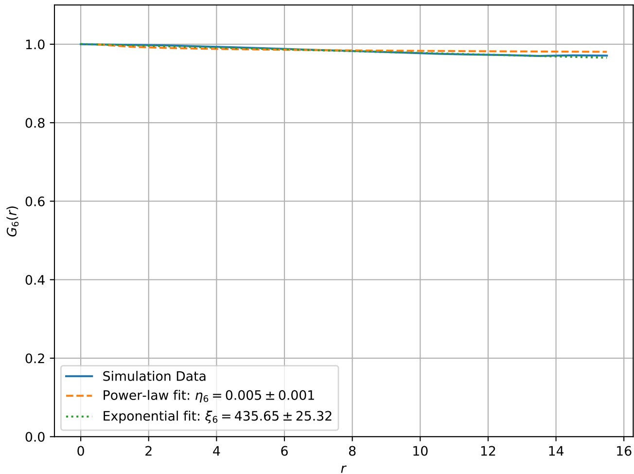
Correlation Function at T = 1.00e - 05 , L = 32
