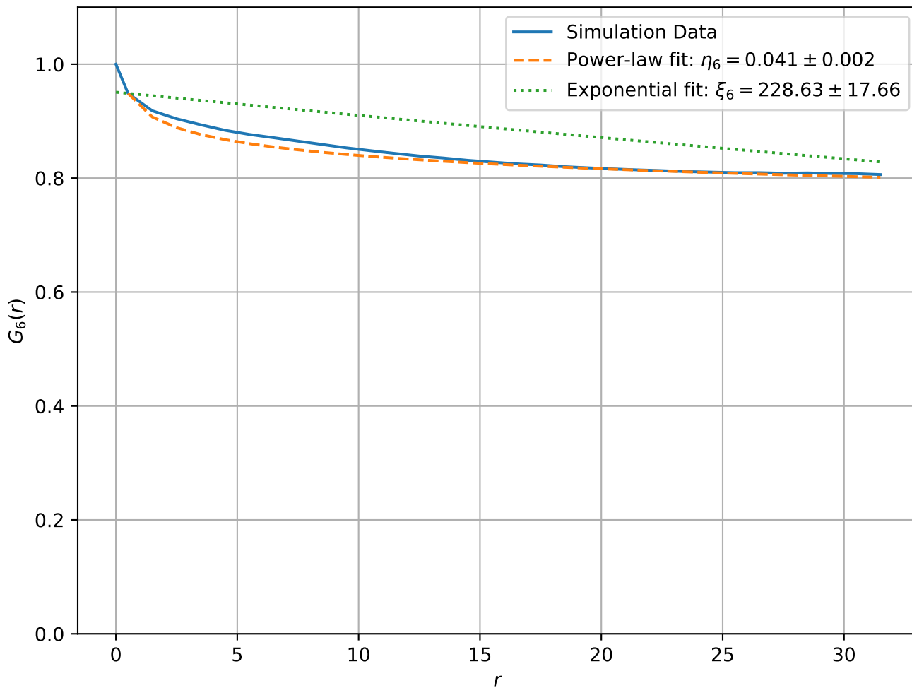
Correlation Function at T = 1.20e - 01 , L = 64
