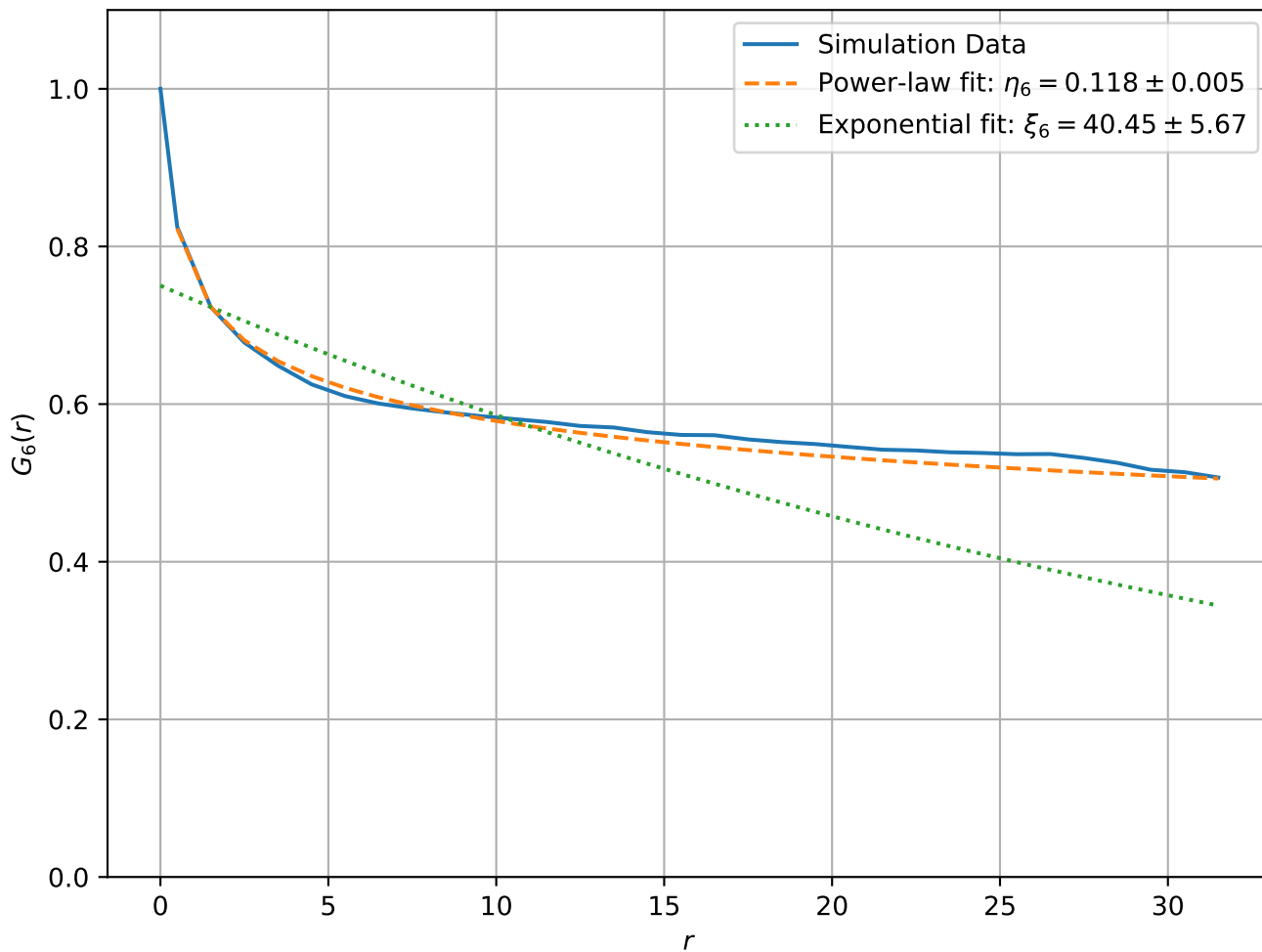
Correlation Function at T = 1.75e - 01 , L = 64
