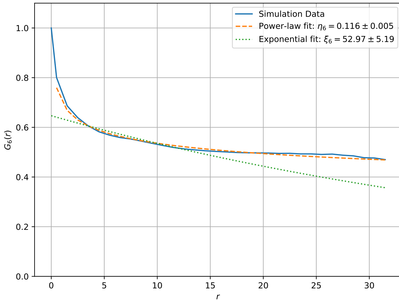
Correlation Function at T = 1.8e - 01, L = 64
