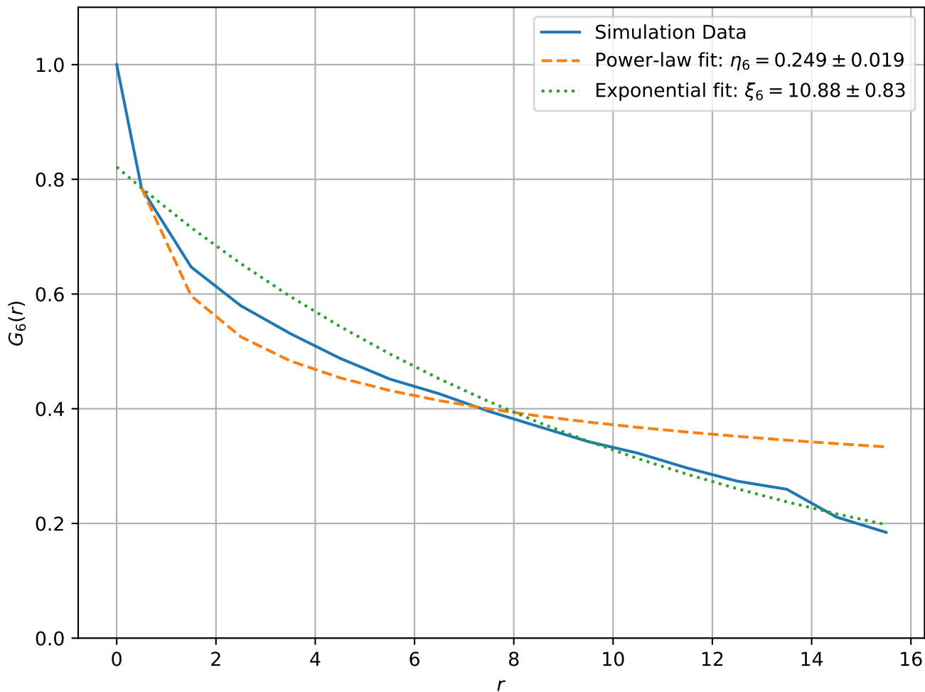
Correlation Function at T = 1.90e - 01 , L = 32
