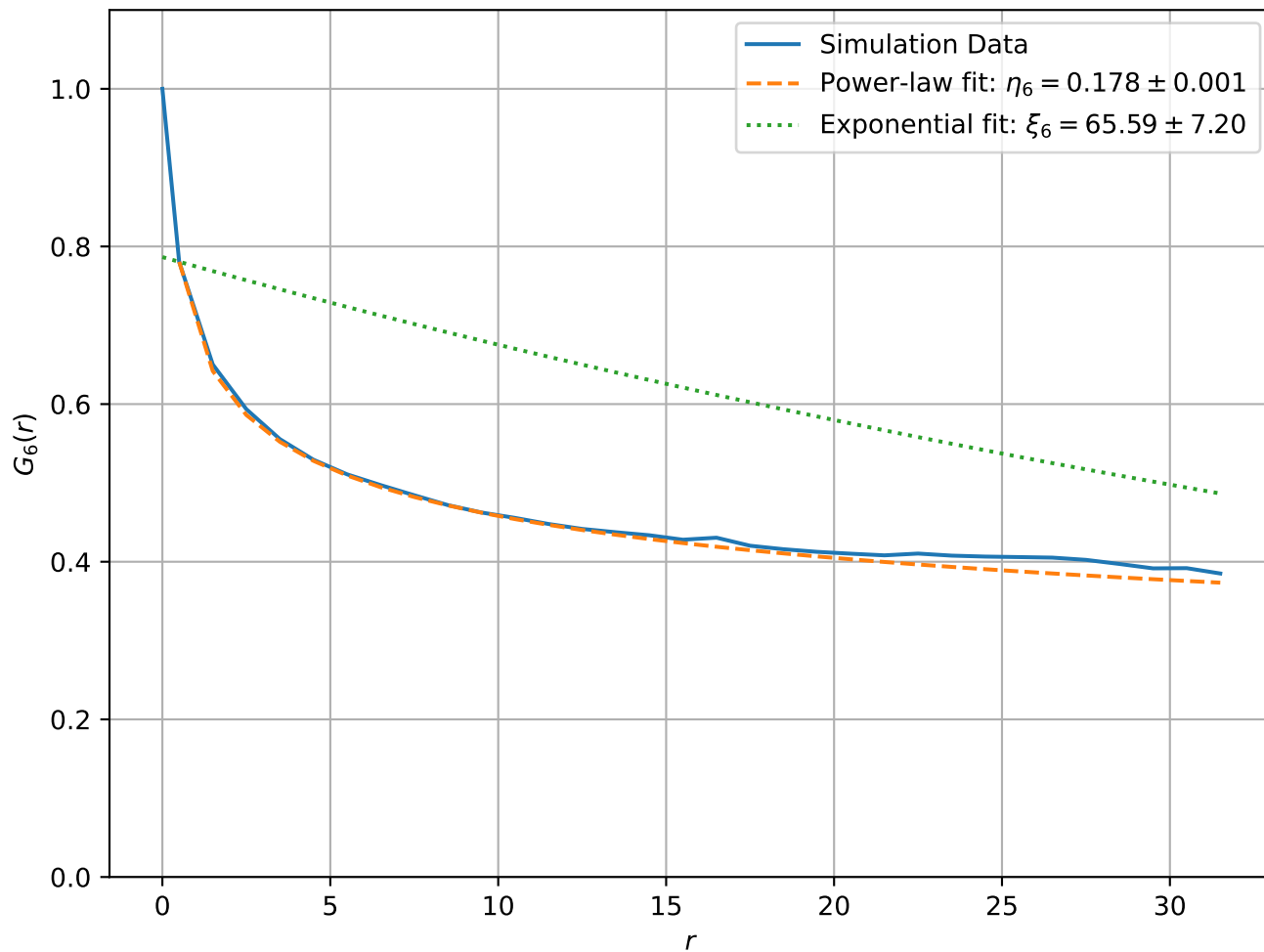
Correlation Function at T = 1.90e - 01 , L = 64
