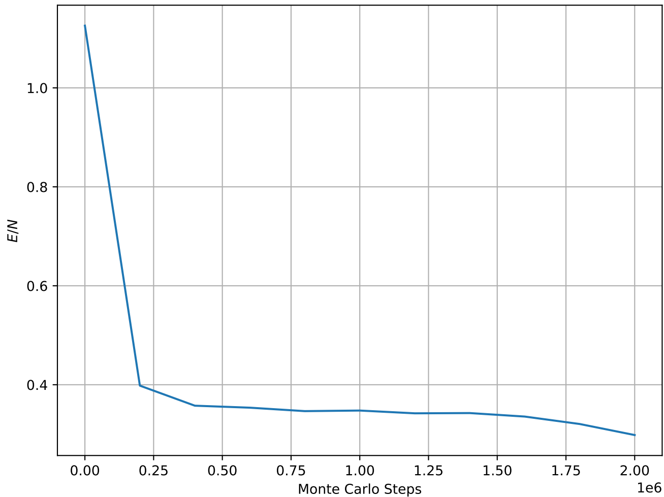
Energy per Spin at T = 1.00e - 01 , L = 64
