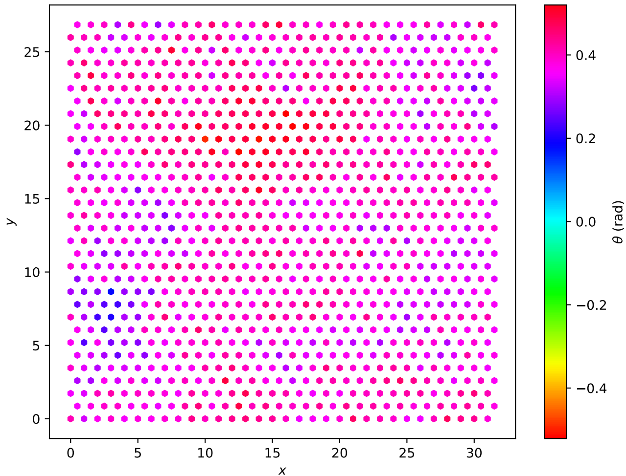
Hexagonal Lattice L=32 , T = 1.00e - 01
