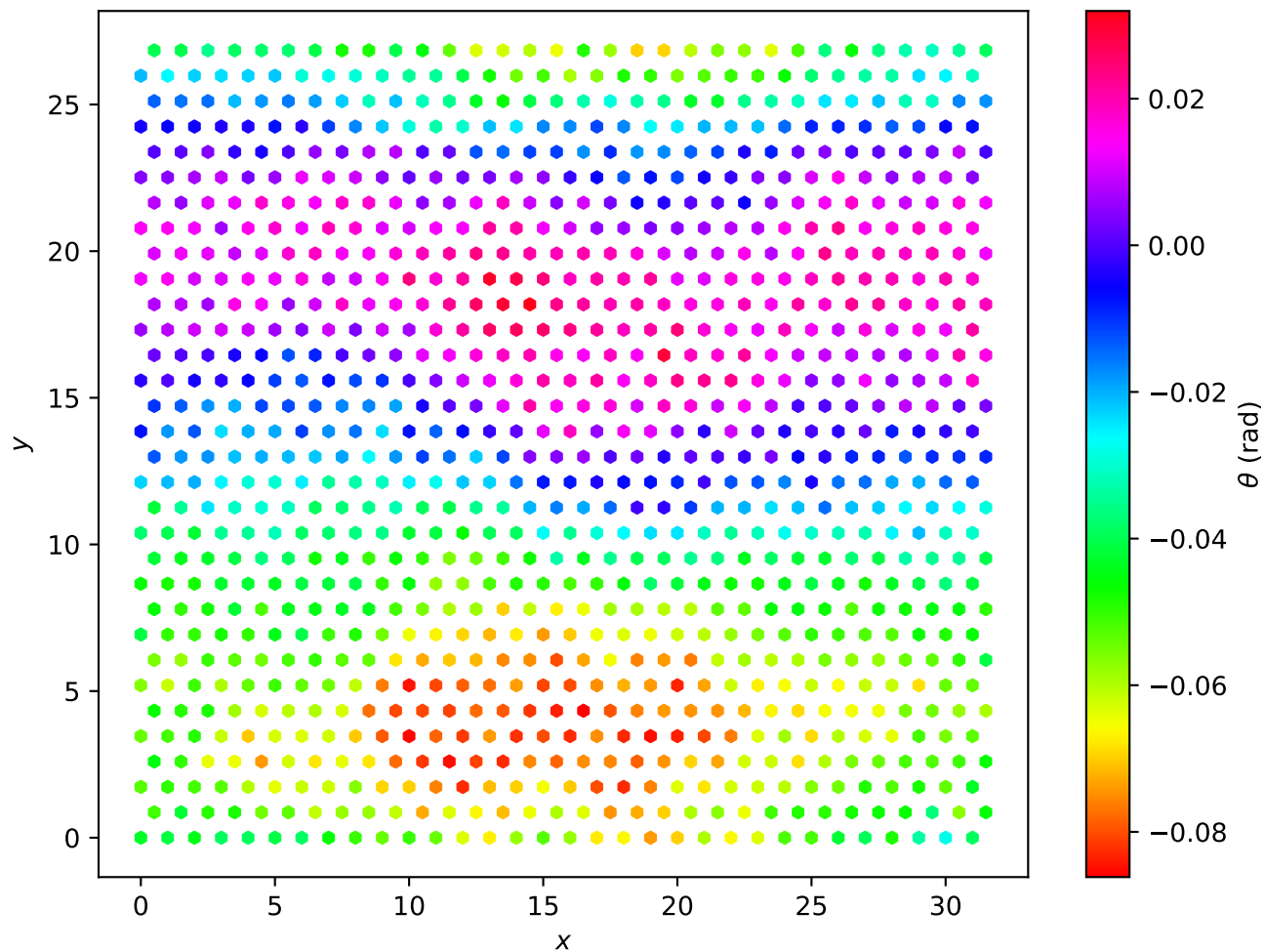
Hexagonal Lattice L=32 , T = 1.00e - 02
