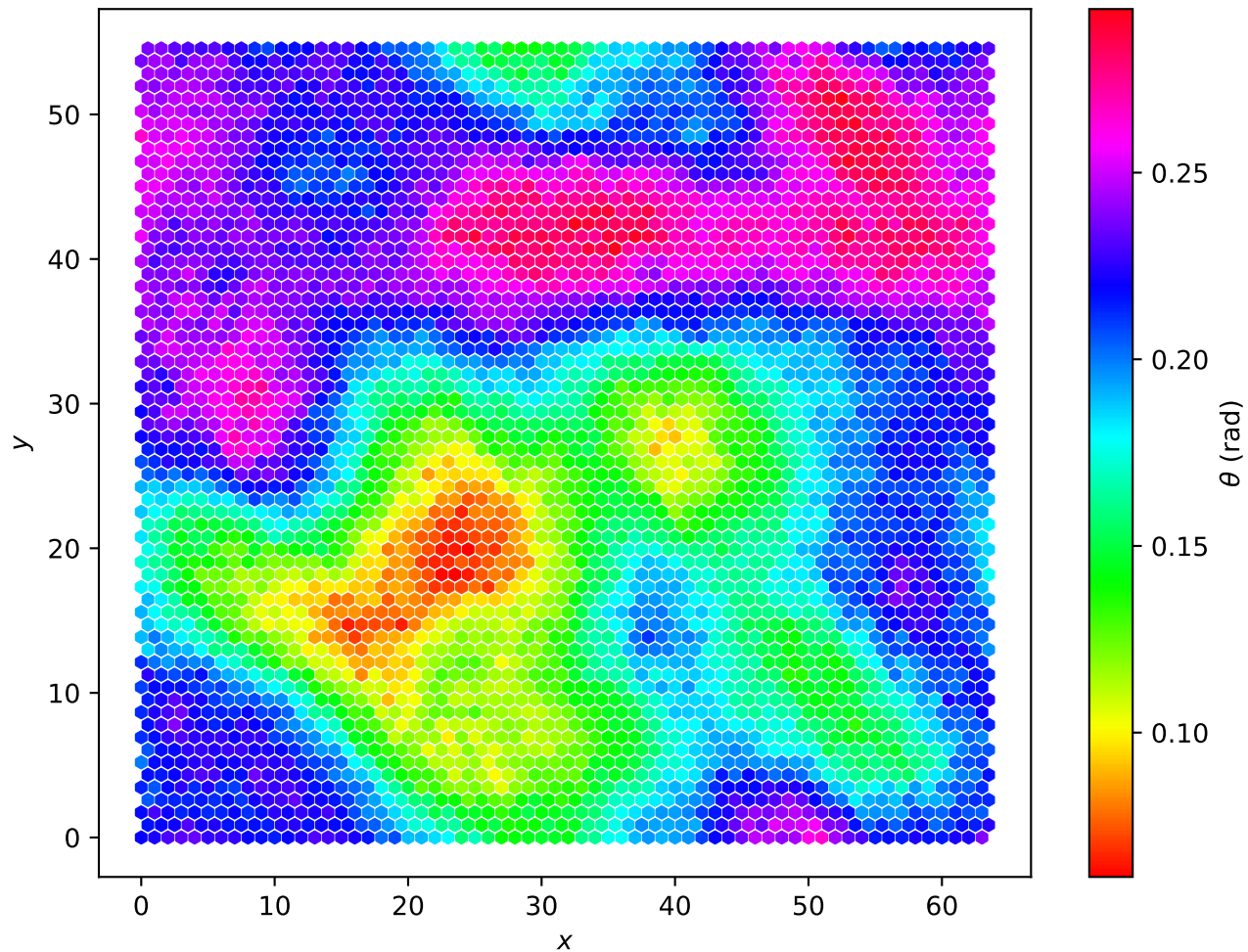
Hexagonal Lattice L=64 , T = 1.00e - 02
