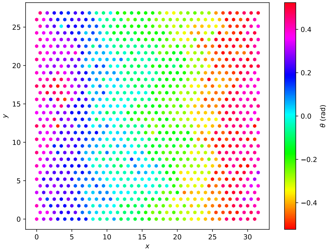
Hexagonal Lattice L=32 , T = 1.20e - 01
