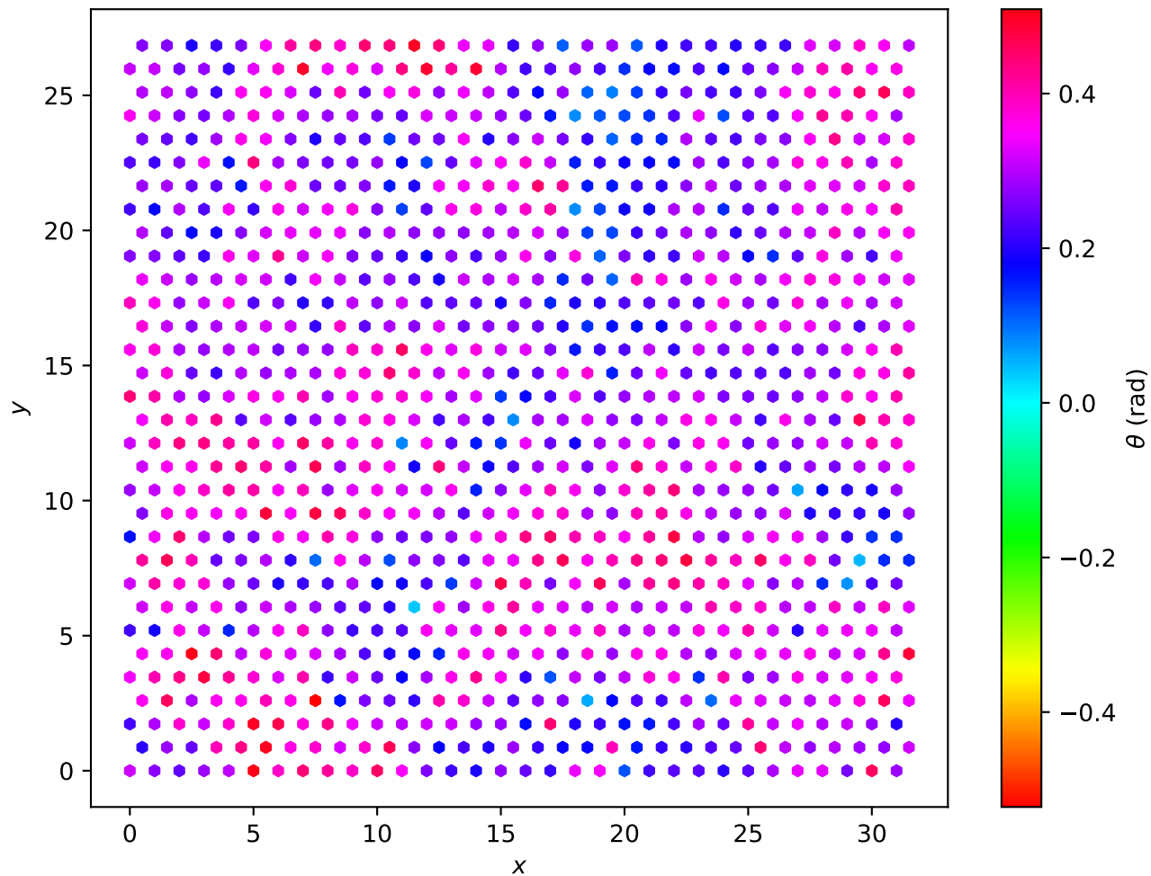
Hexagonal Lattice L=32 , T = 1.50e - 01
