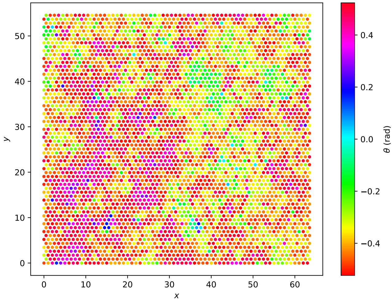
Hexagonal Lattice L=64 , T = 1.75e - 01
