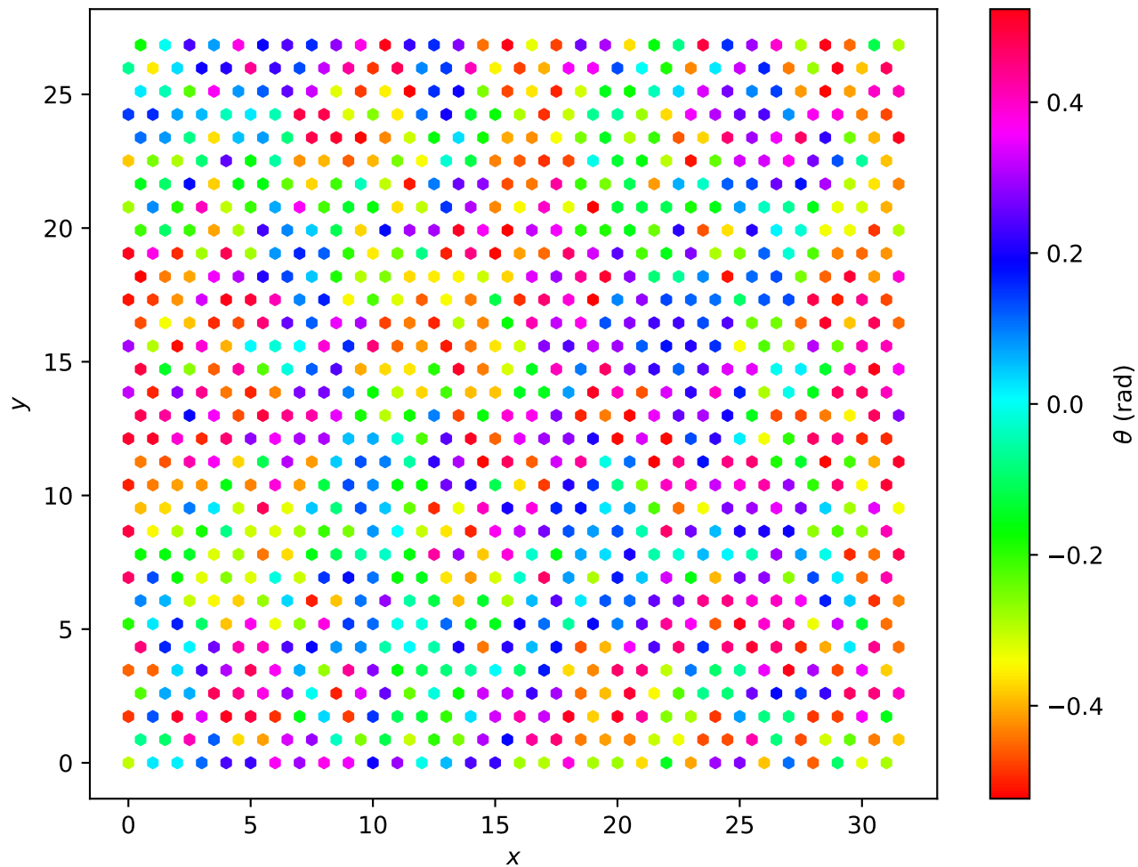
Hexagonal Lattice L=32 , T = 2.50e - 01
