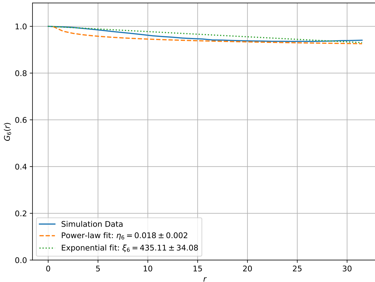
Correlation Function at T = 1.00\text{e} - 05 , L = 64
