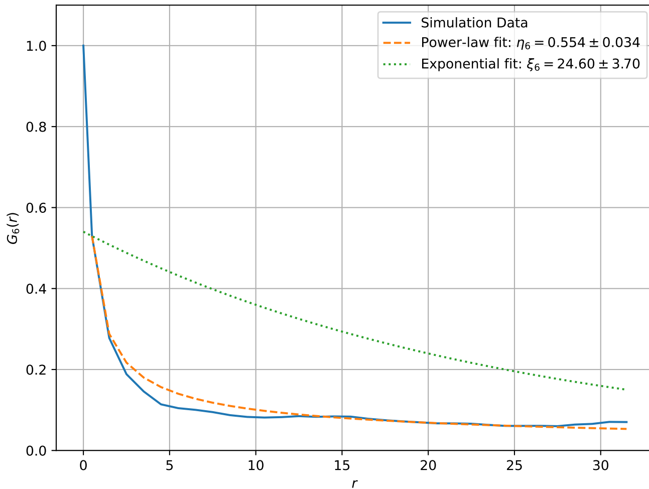
Correlation Function at T = 1.50e - 01 , L = 64
