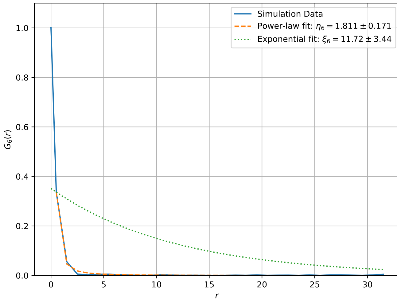
Correlation Function at T = 2.50e - 01 , L = 64
