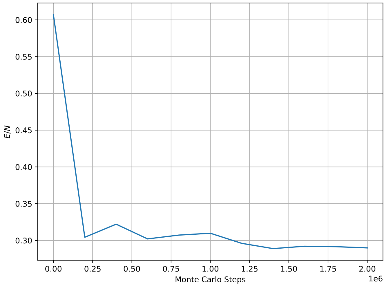
Energy per Spin at T = 1.00e - 01 , L = 64
