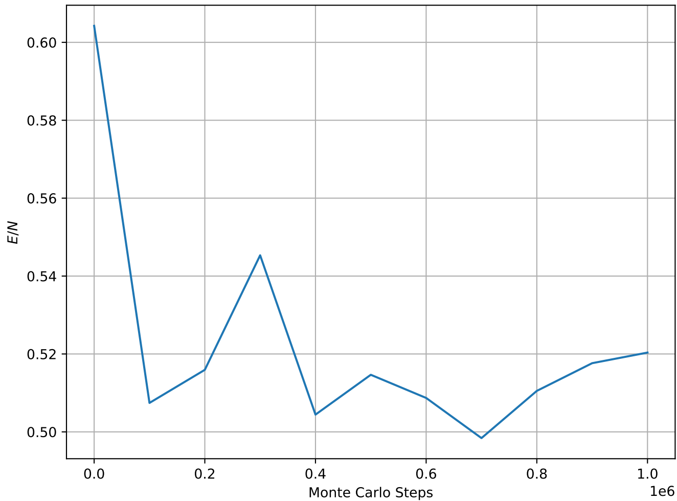
Energy per Spin at T = 2.00e - 01 , L = 32
