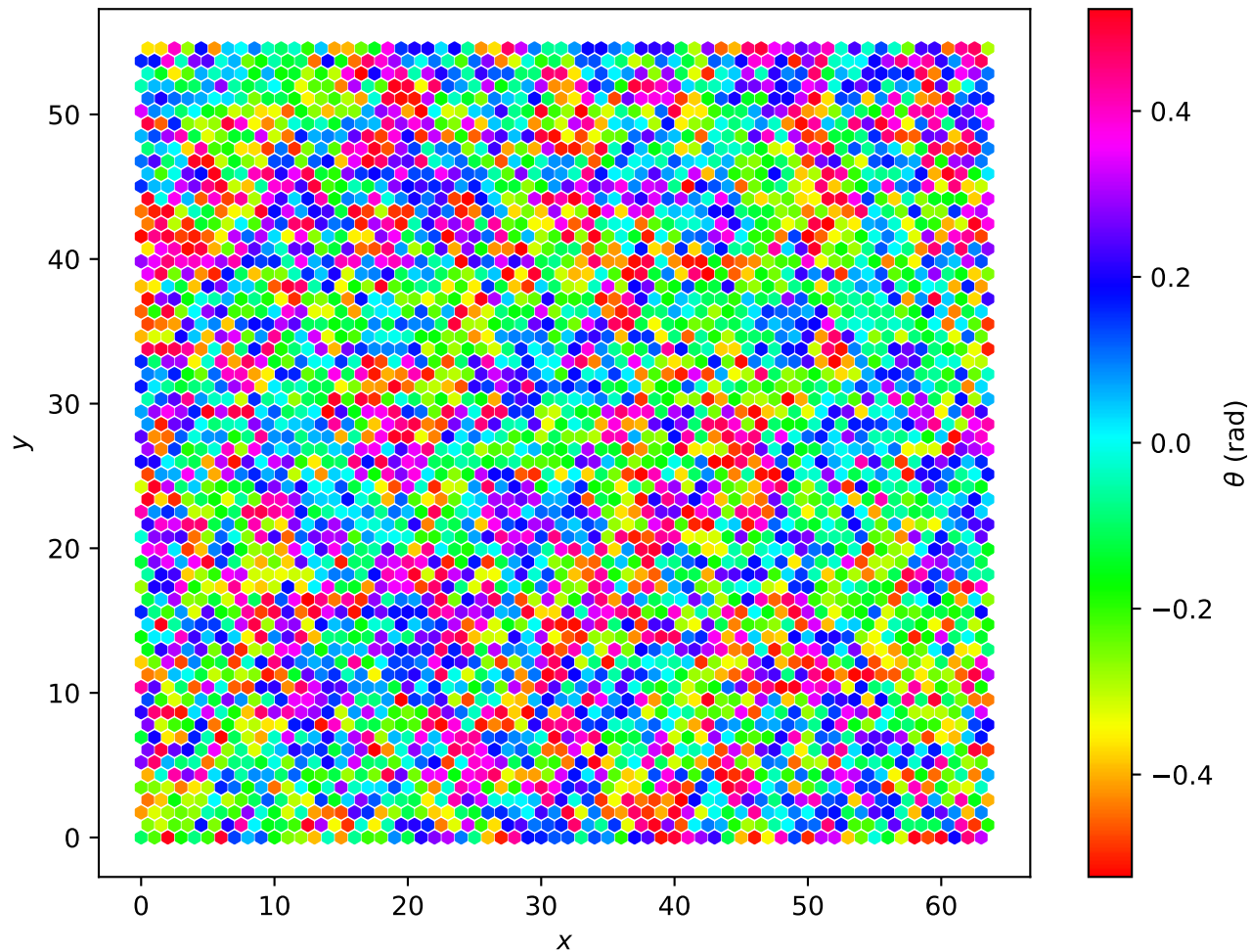
Hexagonal Lattice L=64 , T = 1.70e - 01
