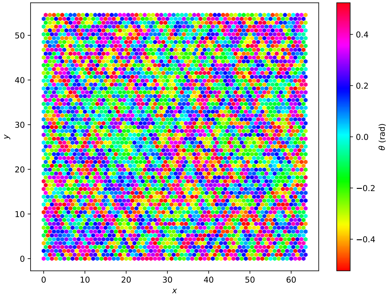
Hexagonal Lattice L=64 , T = 2.00e - 01
