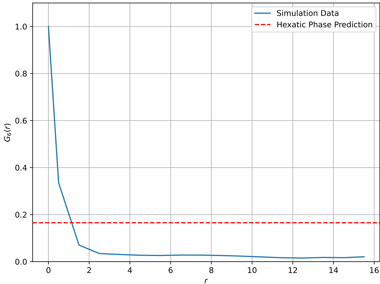
Correlation Function at T = 1.00e - 01 , L = 32
